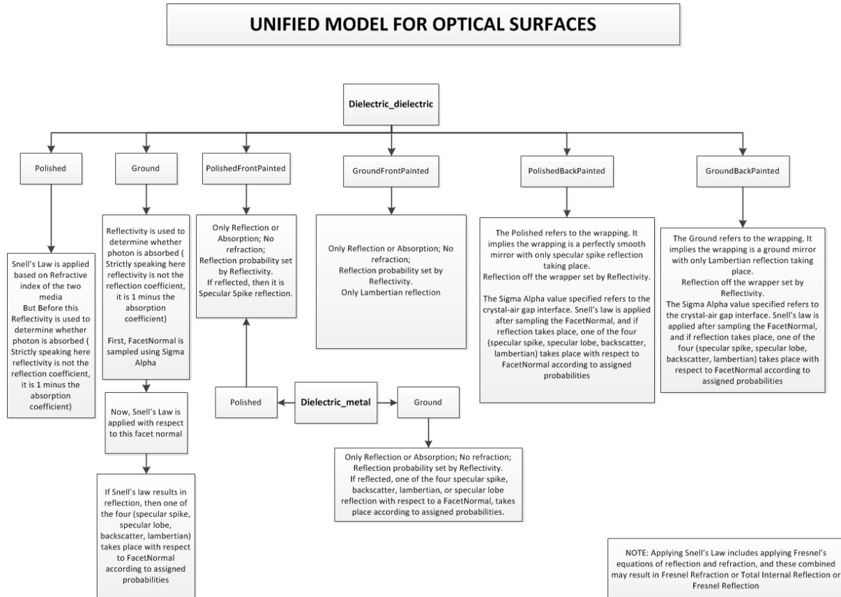
Figure 5.1. Diagram of the UNIFIED Model for Optical Surfaces (courtesy A. Shankar)
