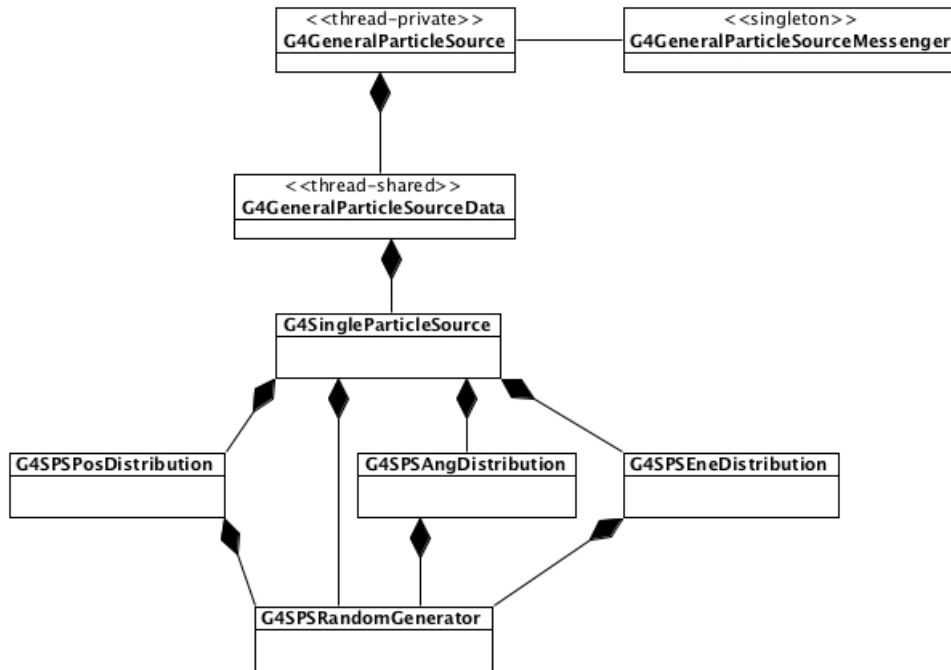
Figure 2.1. The class diagram of G4GeneralParticleSource .
