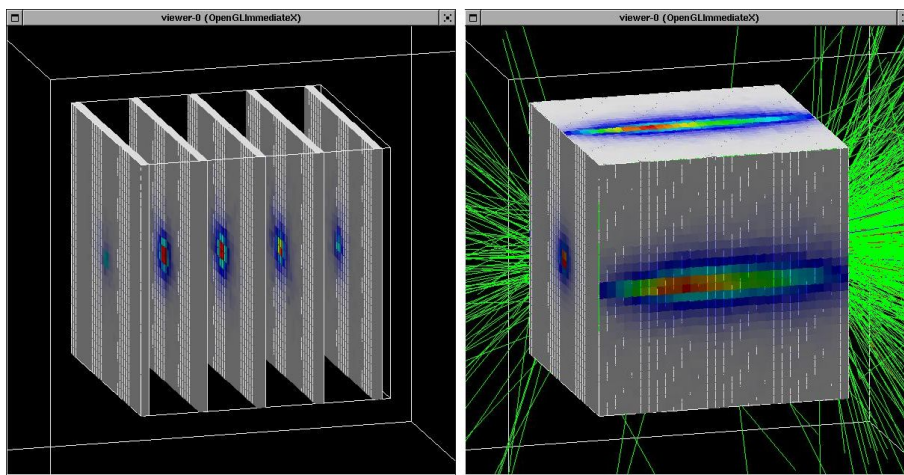
Figure 4.9. Drawing scores in slices (left) and projection (right)
