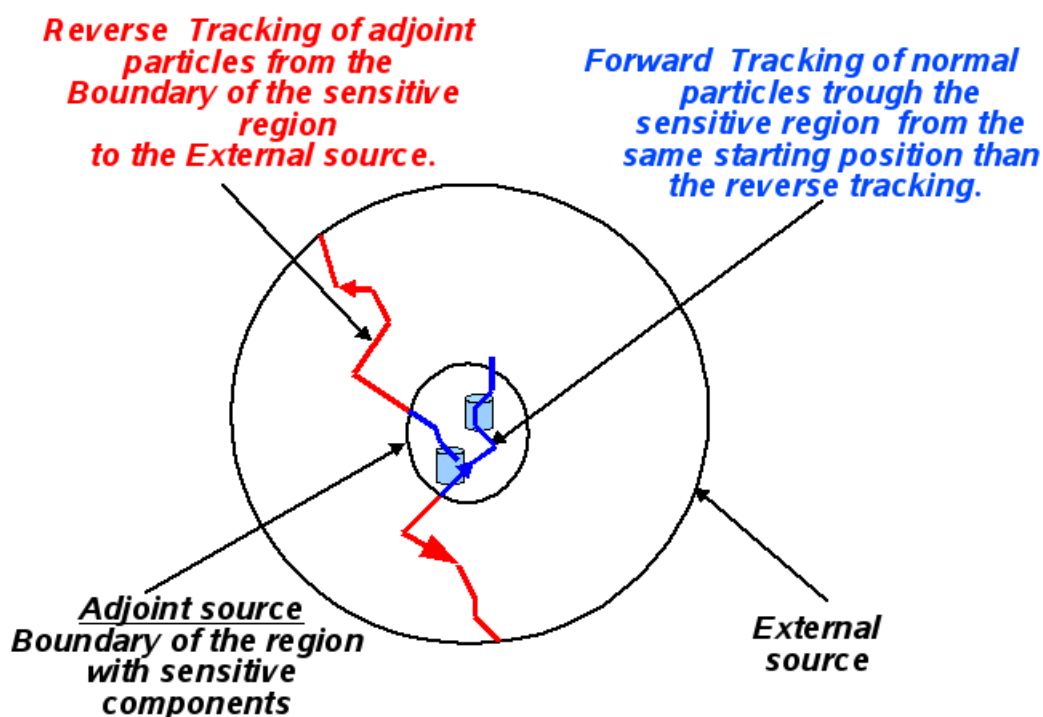
Figure 3.3. Schematic view of an adjoint/reverse simulation in Geant4
